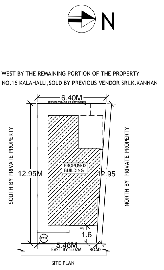
SITE PLAN
